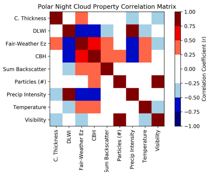
Fig. 7. Correlation matrix of the diurnal variability of 9-explored polar night properties: cloud thickness (c. thickness), downwelling longwave irradiance (DLWI), fair-weather E_z , cloud base height (CBH), sum of vertical backscatter (sum backscatter), number of precipitation particles (particles (#)), precipitation intensity, temperature, and visibility. All correlations that are between plus or minus 0.25 are shown as white, as they are less significant.
