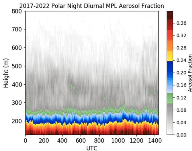
Fig. 3. Two-Dimensional histogram of polar night aerosol occurrence (%) in Barrow, Alaska measured by the Micro Pulse Lidar (MPL). A threshold of 100 \text{ km}^{-1}\text{sr}^{-1} was used to determine the presence/absence of an aerosol event.
