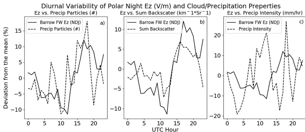
Fig. 4. a) Diurnal variation of the polar-night averaged fair weather electric field (solid), and polar night cloud precipitation particle counts (dashed) measured with the impact distrometer. b) Diurnal variability of the polar-night averaged fair weather electric field (solid), and polar night cloud sum of vertical column backscatter (dashed) measured with the micro-pulse Lidar. c) Diurnal variability of the polar-night averaged fair weather electric field (solid), and polar night cloud precipitation intensity (dashed) measured with the impact distrometer. All values are normalized as a percent deviation from the mean value during polar night in Barrow AK for the years of 2017–2021.
