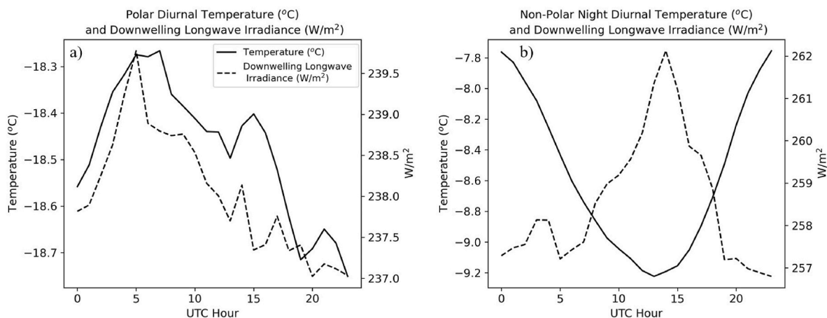
Fig. 6. Diurnal variation of the polar night (a) and non-polar night (b) surface air temperature (solid) and downwelling longwave irradiance (dashed) measured by the SKYRAD during the years of 2017–2022.
