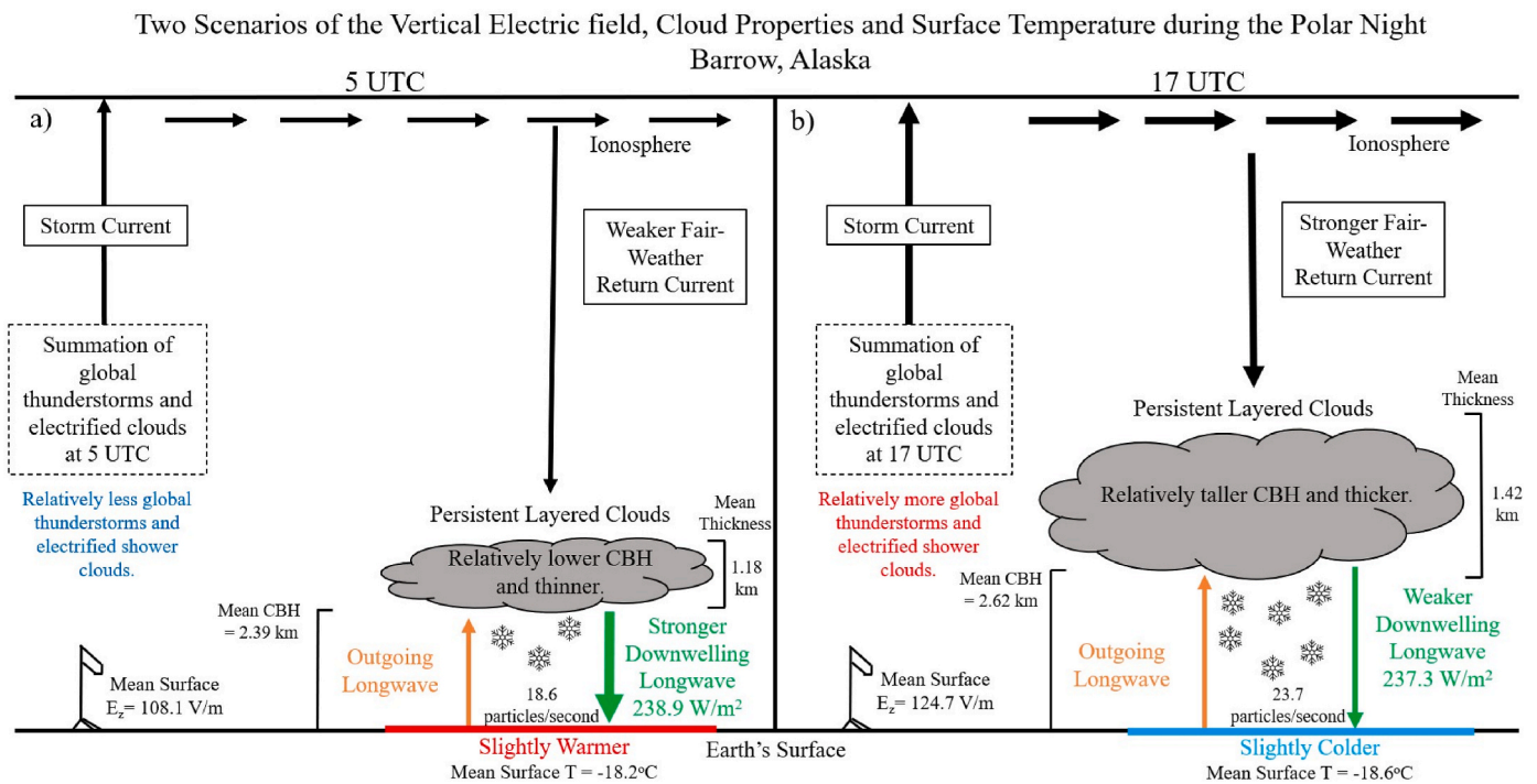
Fig. 8. Summary schematic of the influence of the GEC on diurnal properties of persistent layered clouds and diurnal variation of surface temperature during the polar night.
