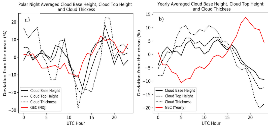
Fig. 1. Diurnal variations of the a) polar-night and b) yearly averaged fair weather electric field (red), cloud-base height (solid), cloud top height (dashed), and cloud thickness (dotted) measured with the Micro-Pulse Lidar (MPL) in Barrow AK during the years of 2017–2022.
